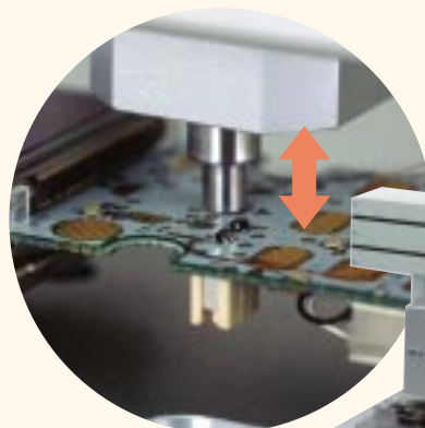
Cycling fatigue test of mounted PCB
